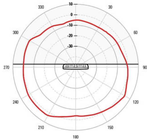
ELEVATION 5 GHZ
