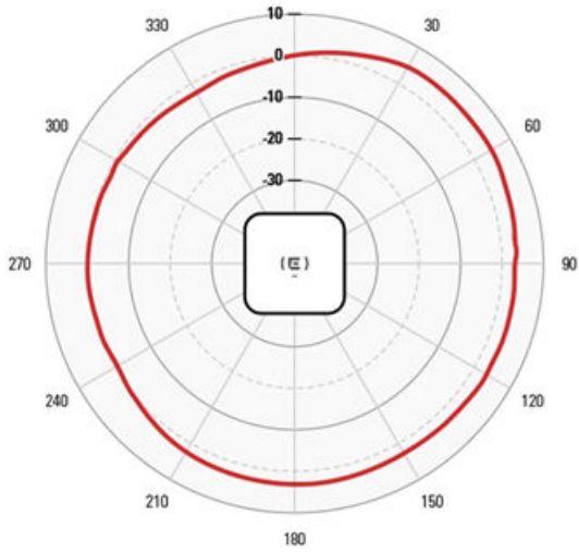
AZIMUTH 5 GHZ
