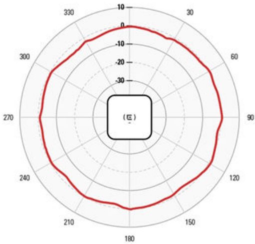
AZIMUTH 5 GHZ
